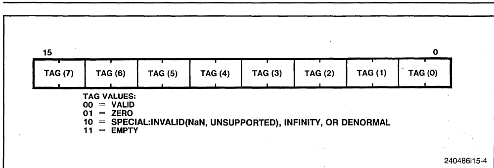
Figure 15-4. Tag Word Format
