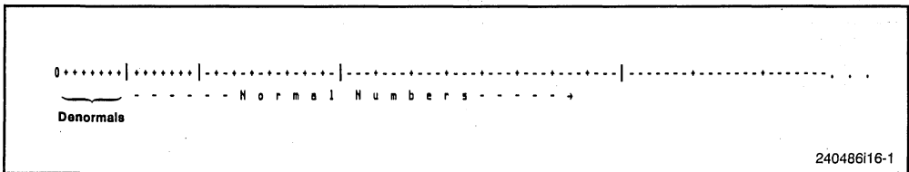
Figure 16-1. Floating-Point System with Denormals
