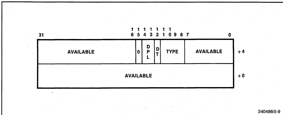
Figure 5-9. Segment Descriptor (Segment Not Present)
