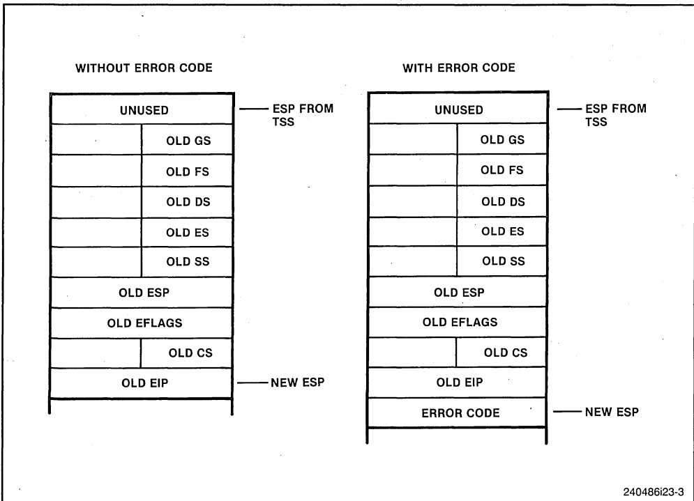
Figure 23-3. Privilege Level 0 Stack After Interrupt in Virtual-8086 Mode
