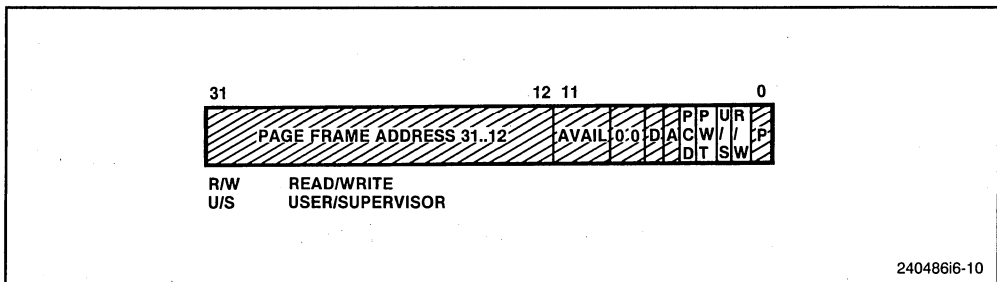
Figure 6-10. Protection Fields of a Page Table Entry
