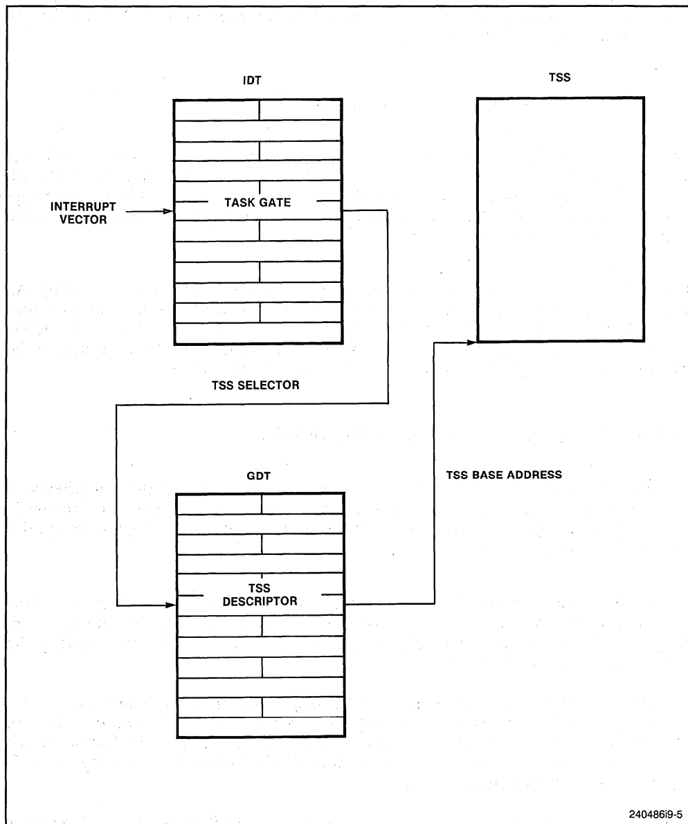
Figure 9-5. Interrupt Task Switch
